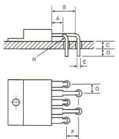
TO-220 Staggered Layover (for 3 thru 23 lead devices)
