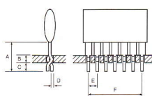
SIP Snap-In Stand-Off
