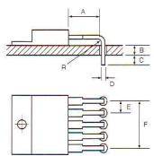
TO-220 In-Line Layover (for 3 thru 23 lead devices)
